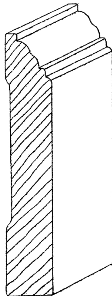
B-90 3/4" X 4-1/2"
