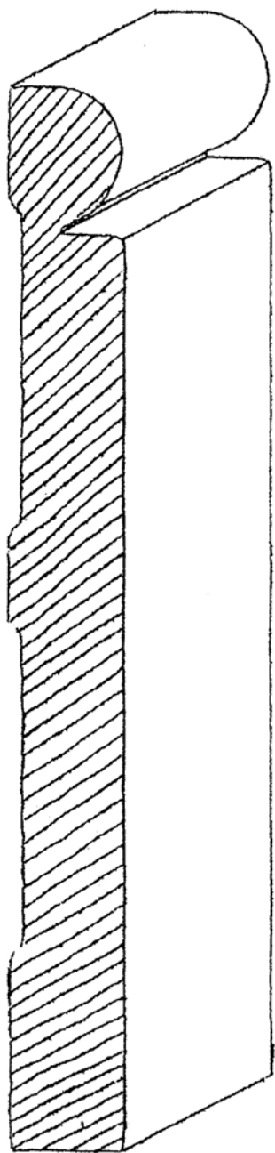
B-67 3/4" X 7-1/4"
