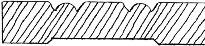
CA-20 3/4" X 2-1/4"
