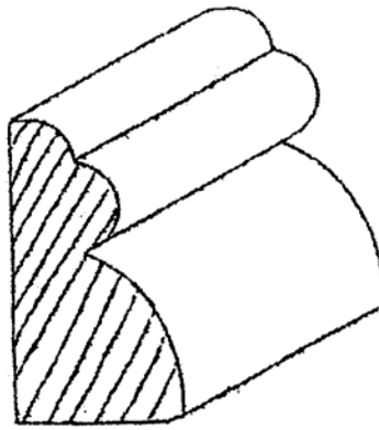
CAP-39 7/8" X 1-1/2"
