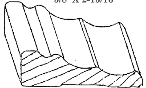
CA-84 5/8" X 2-15/16"
