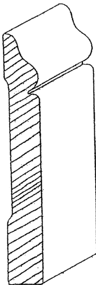
B-58 5/8" X 4-1/2"
