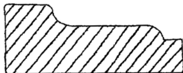
CA-26 3/4" X 1-7/8"
