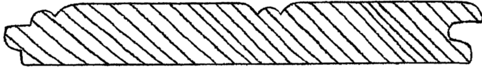
PAN-2 5/8" X 5"
