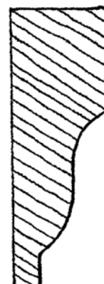
BRICK-3 11/16" X 2"
