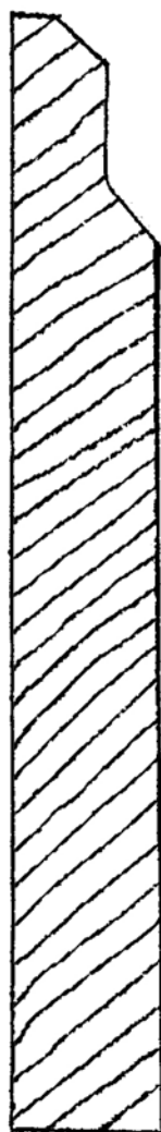
B-21 3/4" X 3-1/2"
