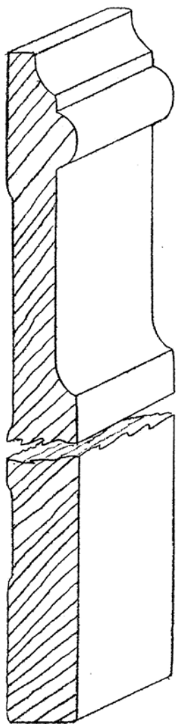
B-87 3/4" X 9-1/4" (max.)
