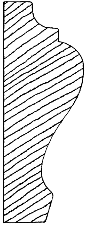
DRIP-20 1-5/8" X 4-1/2"
