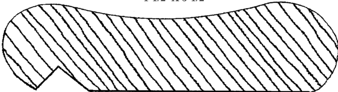
BR-4 1-1/2" X 5-1/2"
