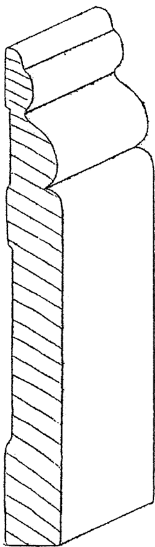
B-45 5/8" X 5-1/2"
