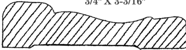
CA-28 3/4" X 3-3/16"
