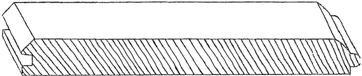
TONGUE & GROOVE V-GROOVE 3/4" X 9" max.
