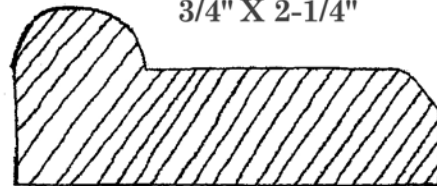
CA-62 3/4" X 2-1/4"
