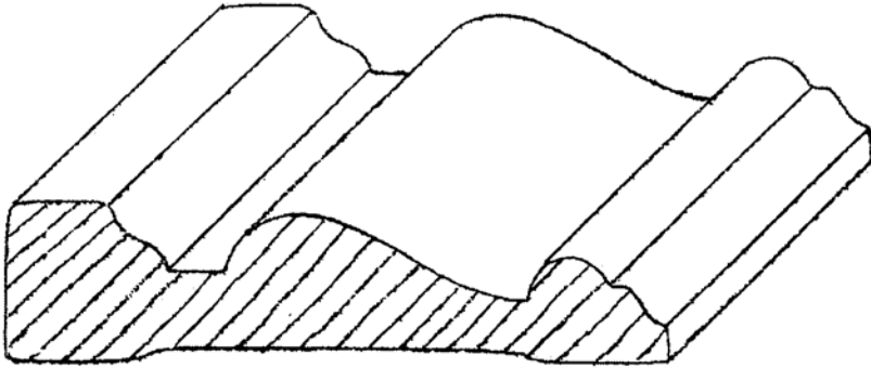
CA-173 13/16" X 3-1/4"
