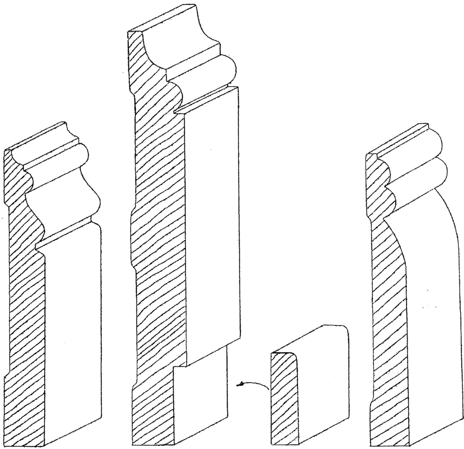
B-49 3/4" X 5-1/2"
