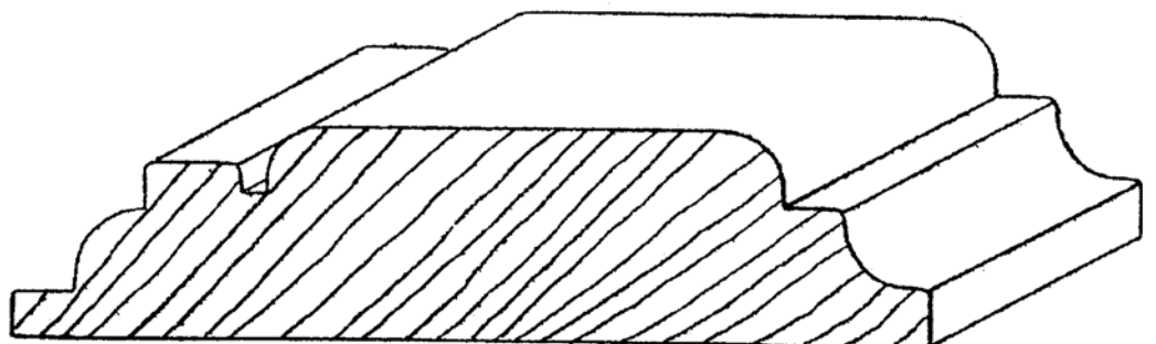
CH-51 1-1/16" X 4-1/2"
