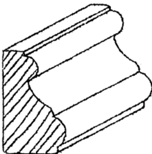
CAP-44 11/16" X 1-1/8"
