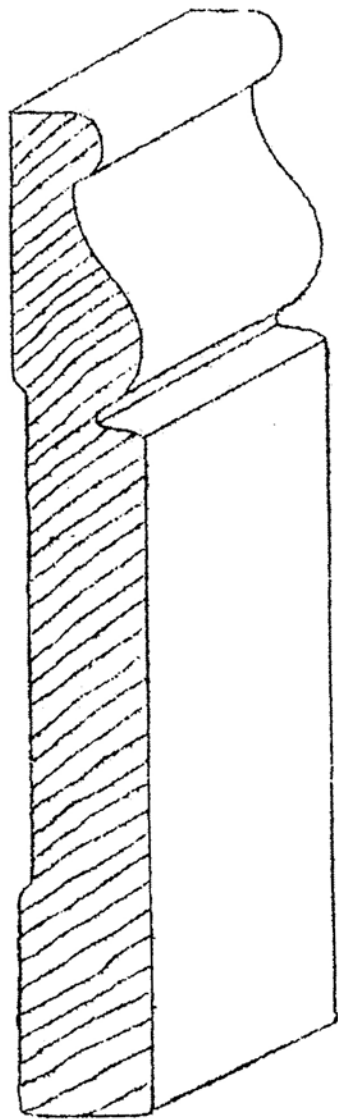
B-75 3/4" X 5-1/2"
