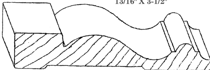
CA-81 13/16" X 3-1/2"
