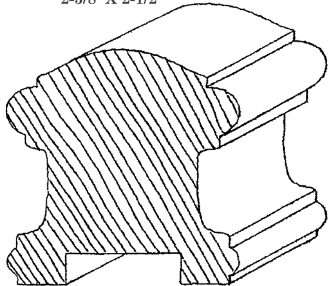
HR-17 2-5/8" X 2-1/2"
