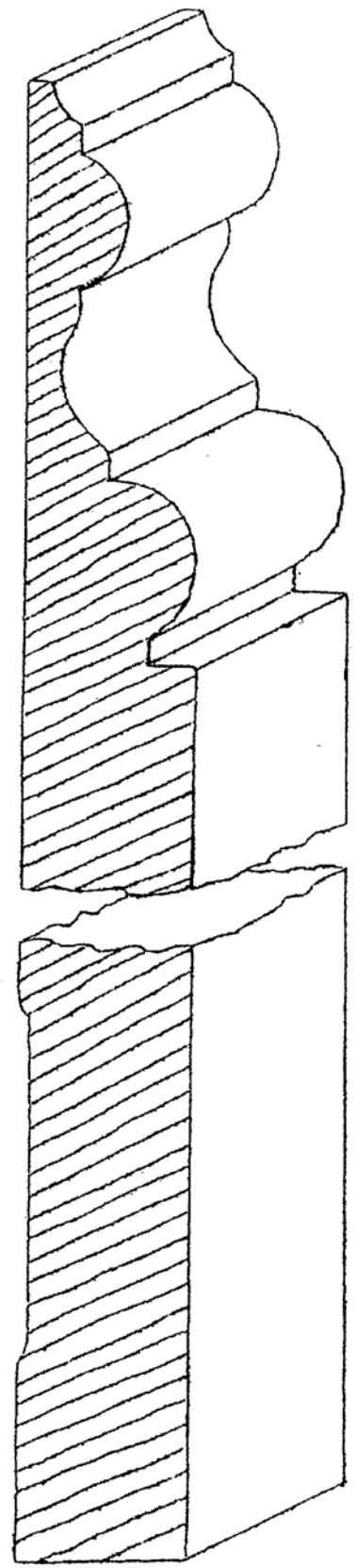
B-62 1-1/8" X 9"
