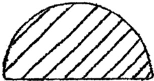
1/2 ROUND 3/4" X 1-1/2"
