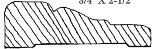
CA-4 3/4" X 2-1/2"
