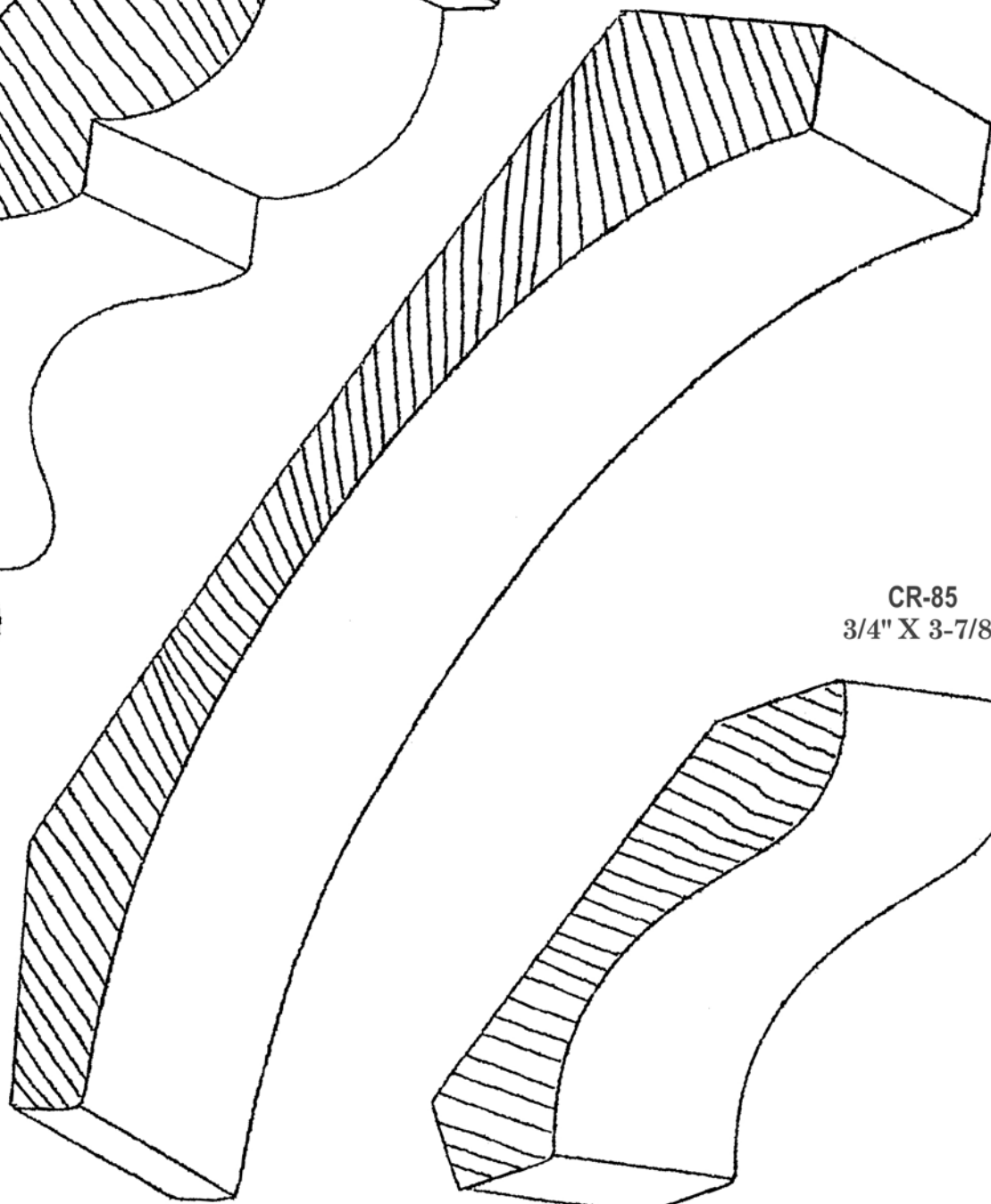
CR-84 1-1/4" X 8-1/4"
