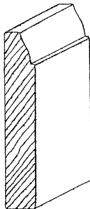
B-106 1/2" X 3-1/4"
