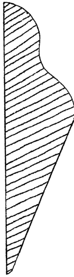
DRIP-24 1-1/4" X 4"
