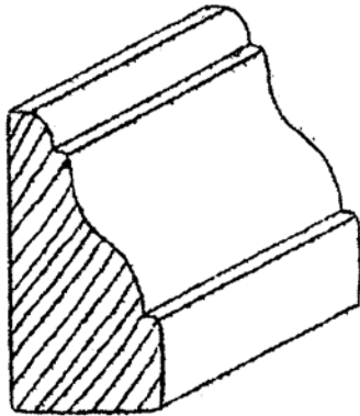
CAP-41 3/4" X 1-1/2"
