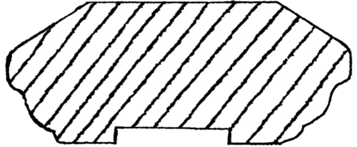
HR-2 1-3/8" X 3-7/16"
