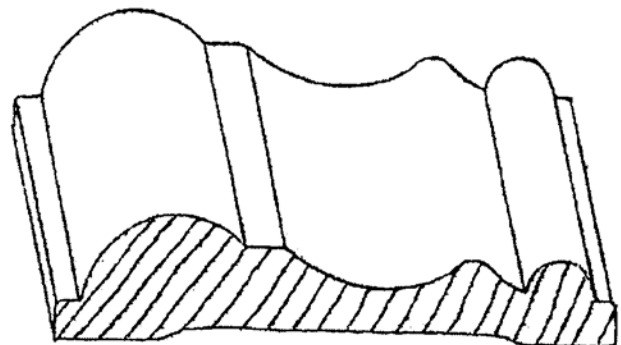
CH-39 5/8" X 3-1/8"
