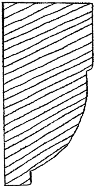
DRIP-1 1-5/8" X 3-1/8"
