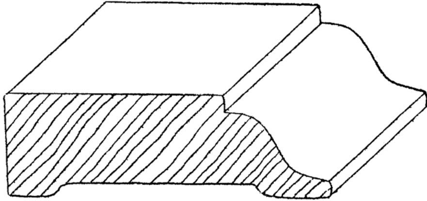
CA-169 1-1/8" X 3-9/16"
