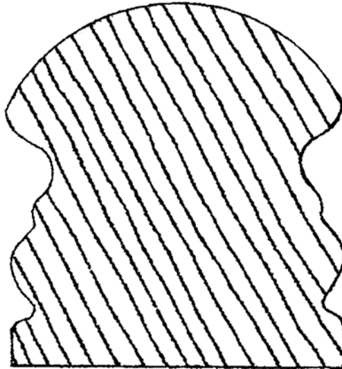
HR-3 2-9/16" X 2-7/8"
