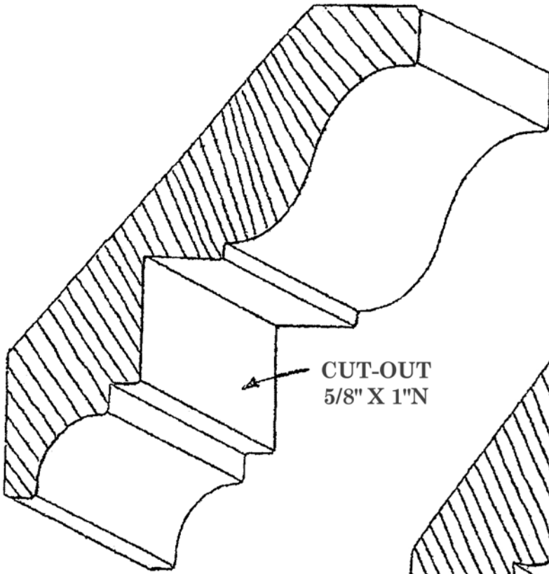
CR-97 7/8" X 5"
