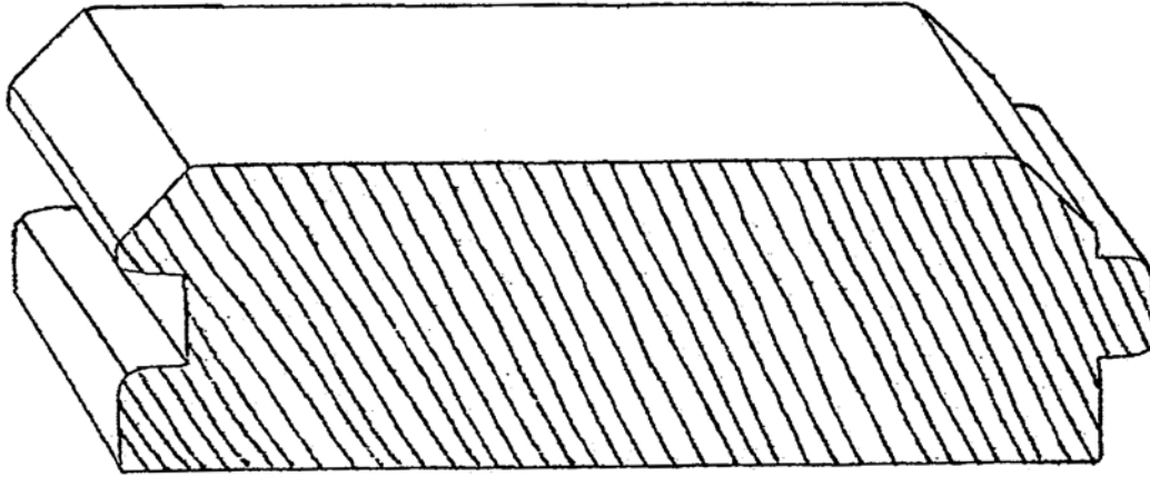
TONGUE & GROOVE V-GROOVE 2" X 9" max.
