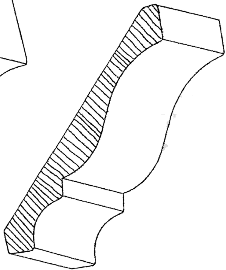
CR-104 3/4" X 3-1/2"
