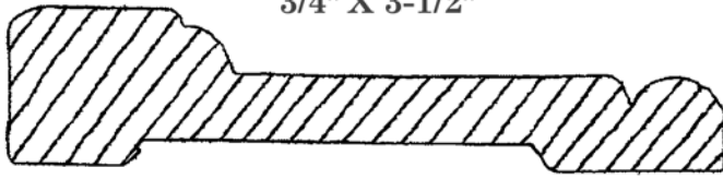
CA-18 3/4" X 3-1/2"
