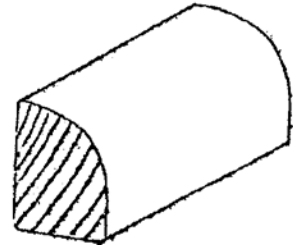
SHOE 1/2" X 3/4"
