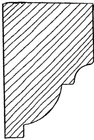
DRIP-11 1-5/8" X 2-3/8"
