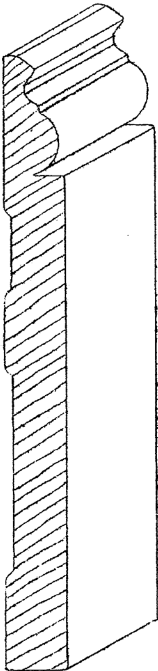
B-83 11/16" X 6-3/4"
