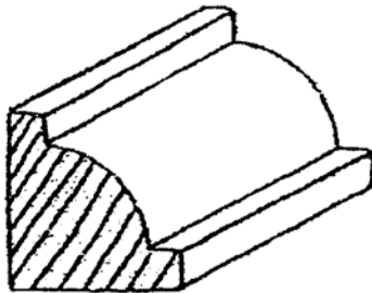
CM-4 7/8" X 7/8"
