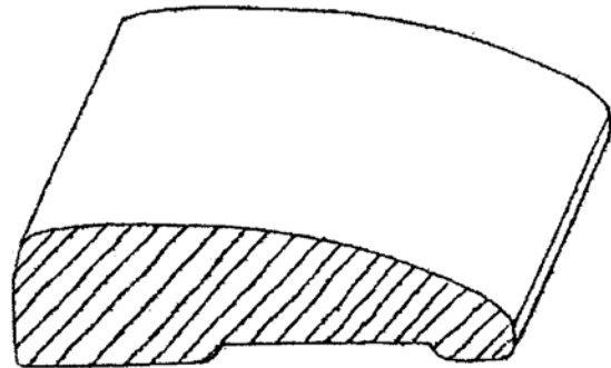
CA-128 11/16" X 2-1/2"
