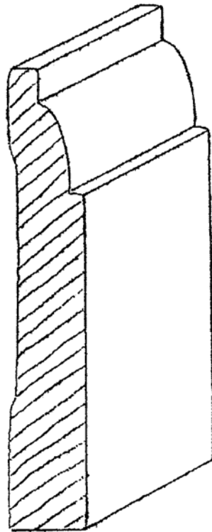
B-80 5/8" X 3-1/2"
