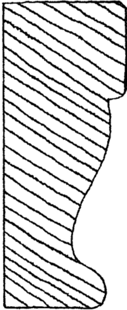
BARGE-1 1-1/4" X 3-1/4"
