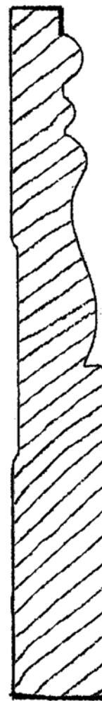
B-6 5/8" X 3" (9" max.)
