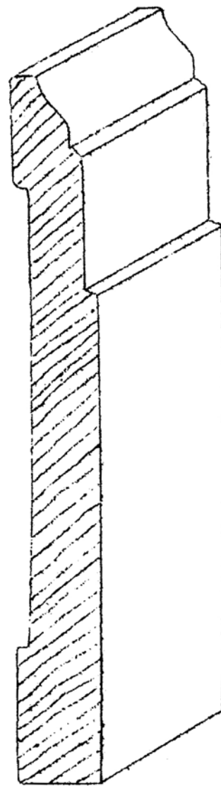
B-78 5/8" X 5-1/2"
