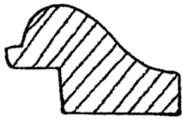
BED MOULD-1 3/4" X 1-1/4"
