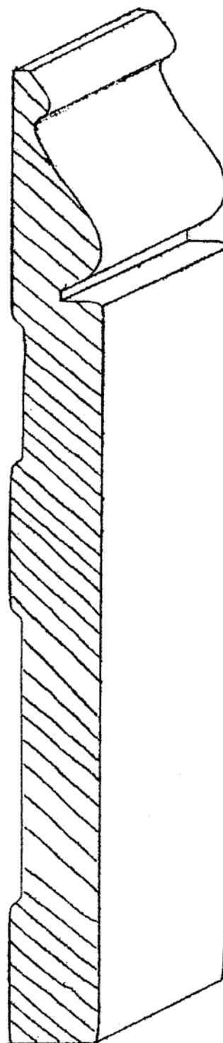
B-44 3/4" X 7-1/2"
