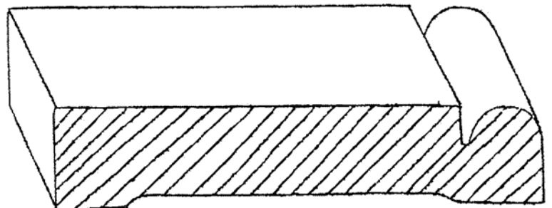
CA-96 3/4" X 3-3/4"
