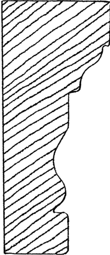
BARGE-2 1-3/4" X 4-1/4"
