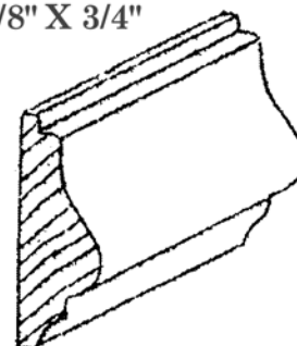
PM-17 3/8" X 3/4"
