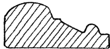
CH-68 1-3/4"
