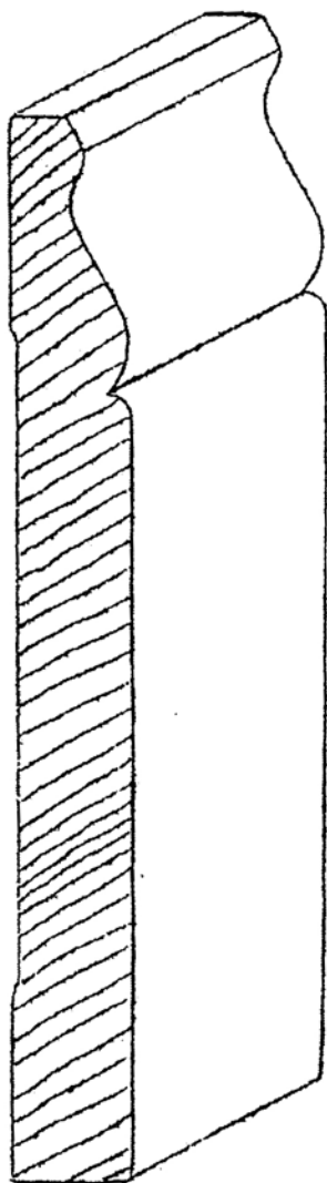
B-71 5/8" X 5-1/4"
