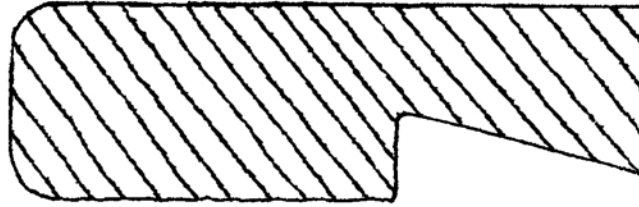
WINDOW SILL-1 1" X 3-1/4"
