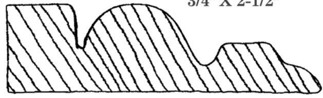
CA-184 3/4" X 2-1/2"
