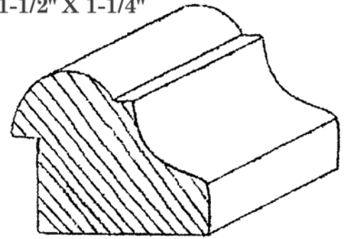
BB-17 1-1/2" X 1-1/4"
