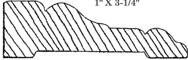
CA-2 1" X 3-1/4"
