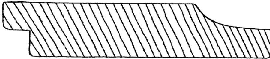
PAN-25 7/8" X 4-1/2"
