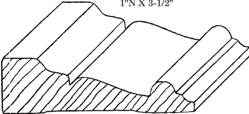
CA-179 1"N X 3-1/2"
