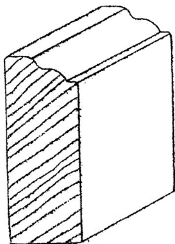
B-100 3/4" X 2"
