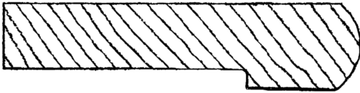
BULLNOSE - 1 15/16" X 9" max.
