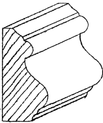
CAP-78 7/8" X 1-3/4"
