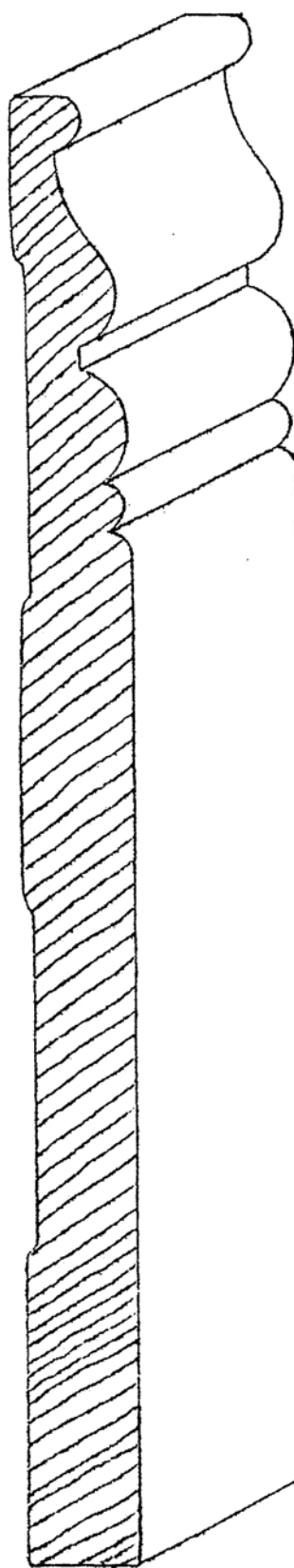
B-47 3/4" X 9-5/16"
