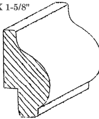
BB-20 1-1/16" X 1-3/4"
