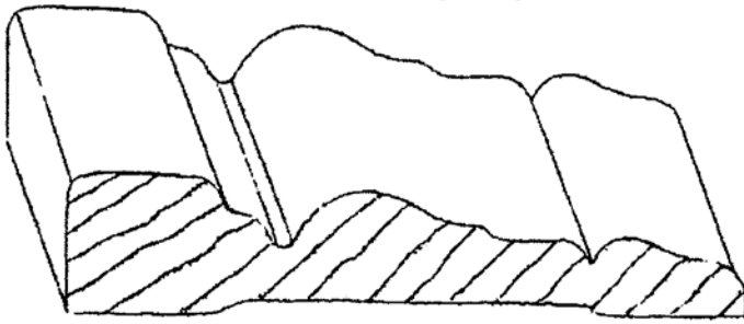
CA-76 11/16" X 3-1/2"
