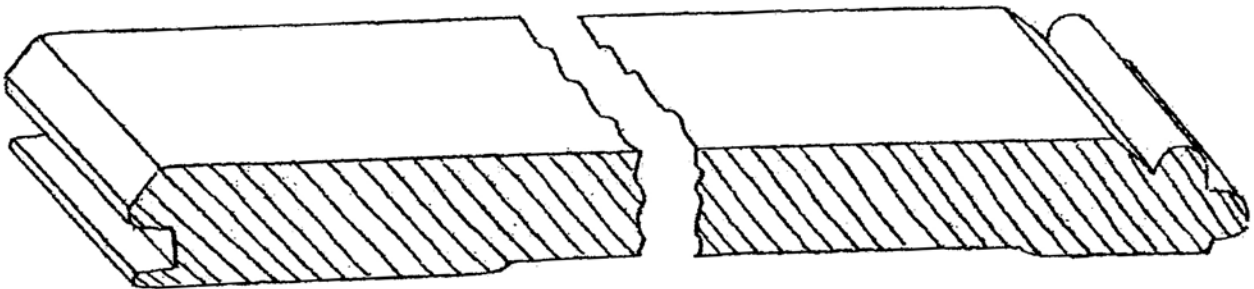
BEADED TONGUE & GROOVE 5/8" X 9" max.
