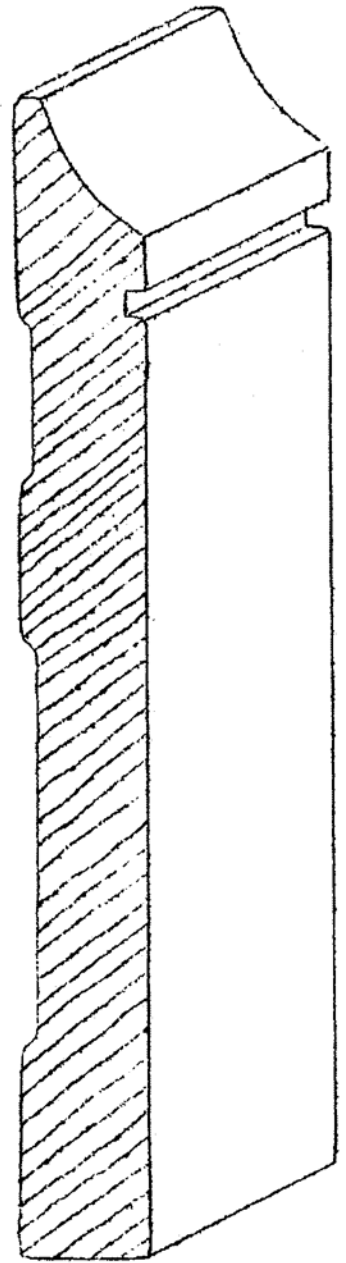
B-82 3/4" X 6-3/8"
