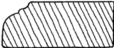
SHELF FRONT-2 3/4" X 1-7/8"
