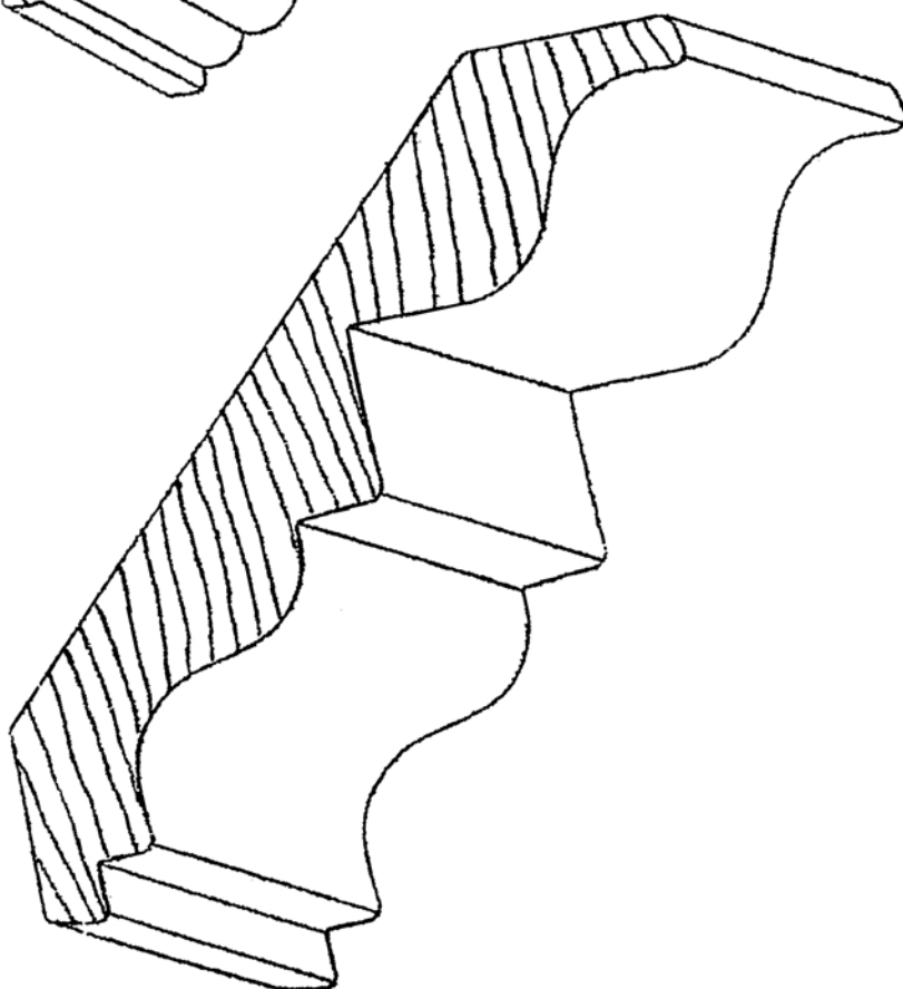
CR-116 13/16" X 5-1/4"
