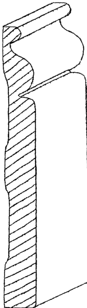
B-39 5/8" X 5-1/2"
