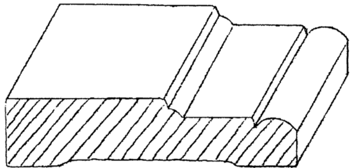
CA-142 3/4" X 3-1/4"
