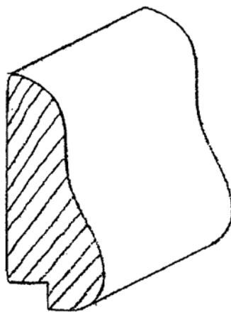
CAP-79 3/4" X 1-3/4"
