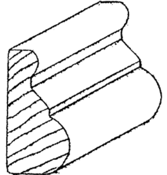
CAP-67 11/16" X 1-3/8"
