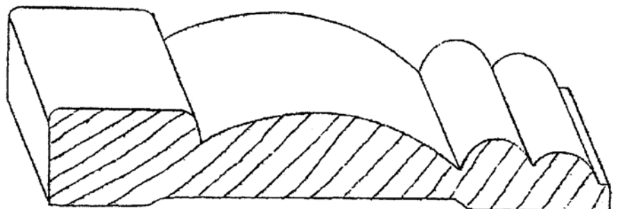
CA-88 3/4" X 4-1/2"
