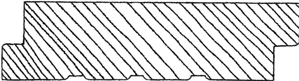
TRUCK FLOOR 1-3/8"
