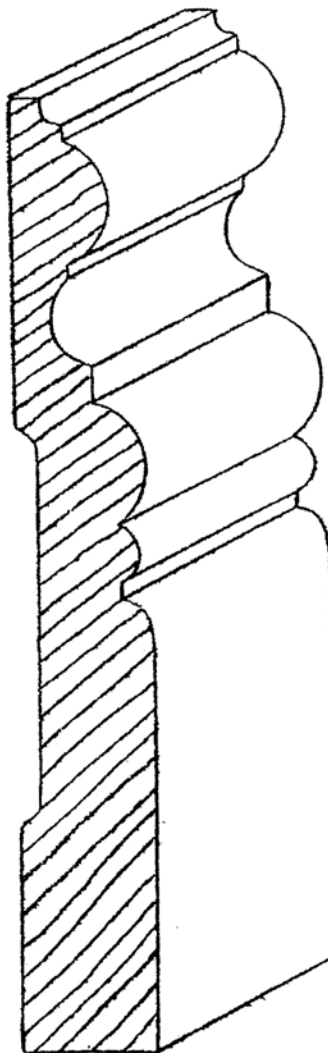
B-89 3/4" X 5-1/2"
