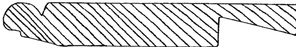
WINDOW SILL-2 3/4" X 4-7/8"
