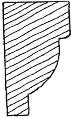
DRIP-6 1-1/8" X 2"
