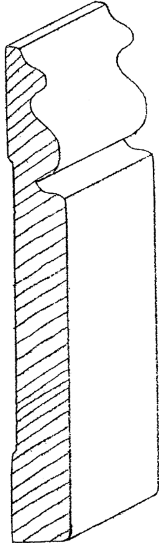
B-86 9/16" X 4-1/2"
