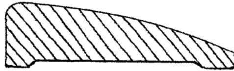
CA-59 5/8" X 2-1/2"
