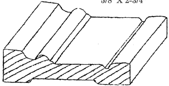
CA-146 5/8" X 2-3/4"
